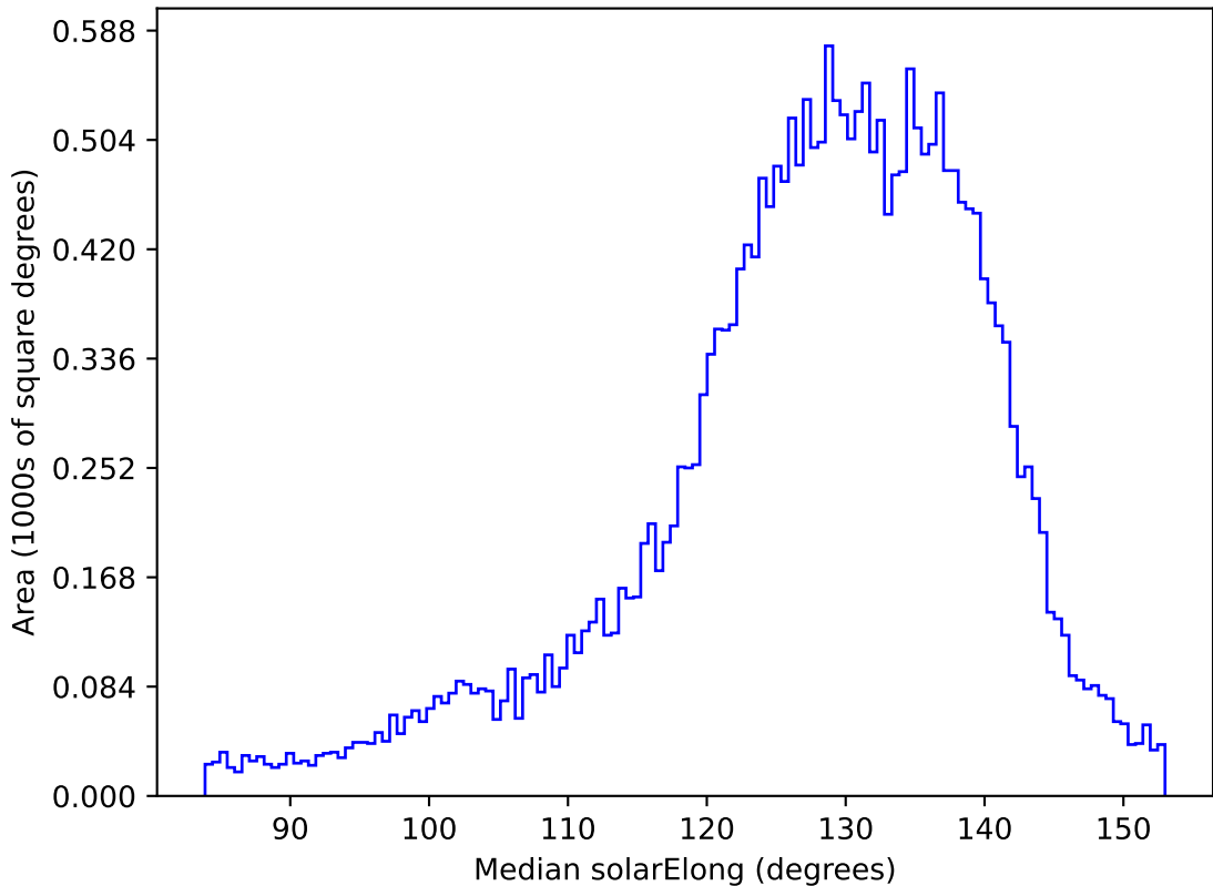
ddf_acor_sf20_lsf0_lsr0_v3.4_10yrs All sky z band: Median solarElong
