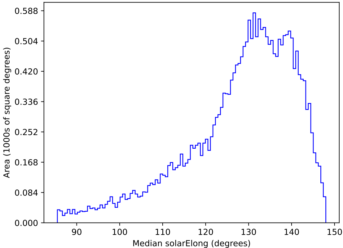
ddf_acor_sf20_lsf0_lsr0_v3.4_10yrs All sky y band: Median solarElong
