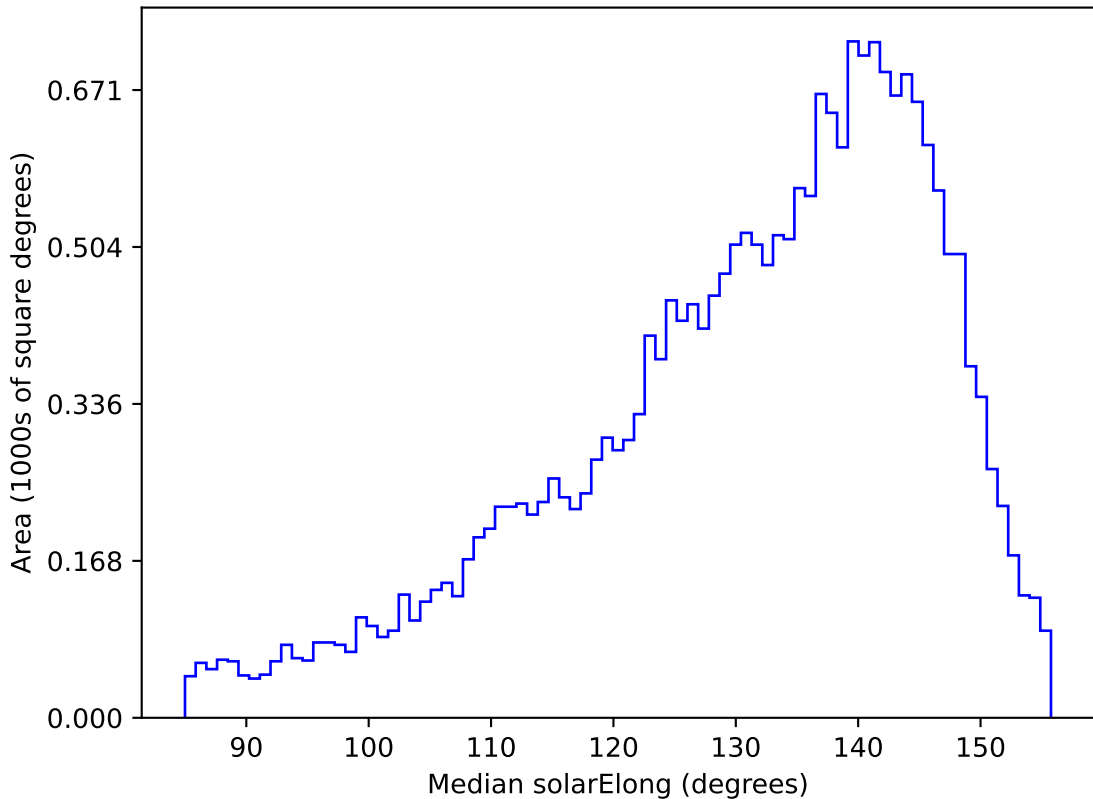
ddf_acor_sf20_lsf0_lsr0_v3.4_10yrs All sky u band: Median solarElong
