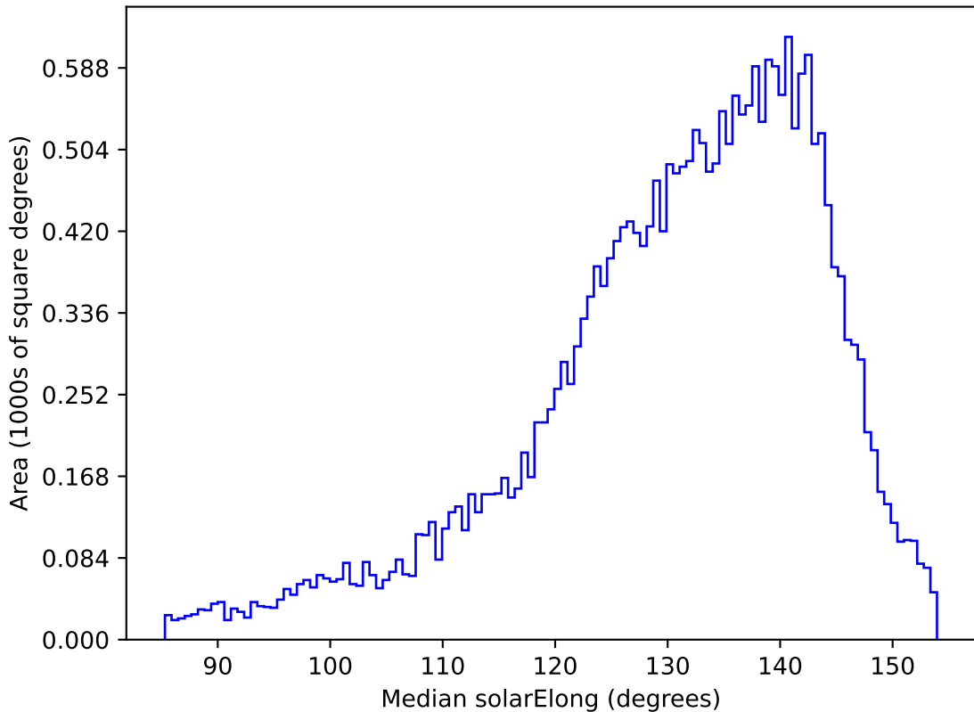
ddf_acor_sf20_lsf0_lsr0_v3.4_10yrs All sky r band: Median solarElong
