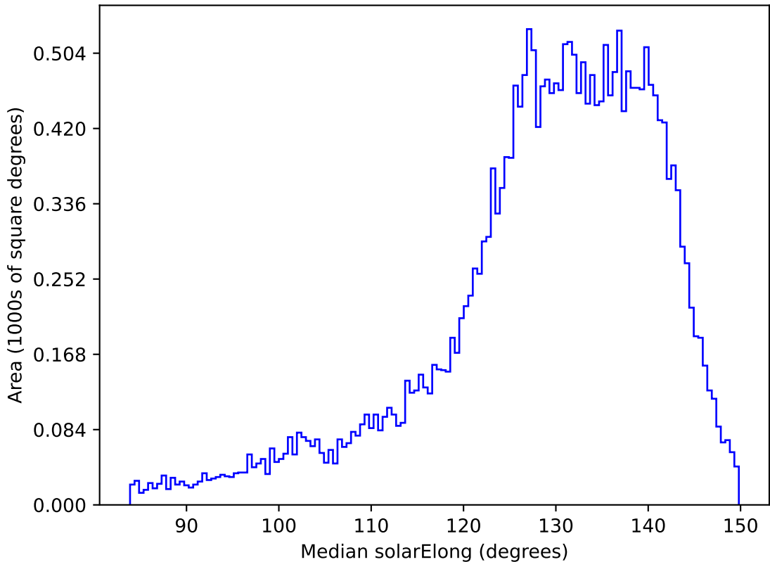
ddf_acor_sf20_lsf0_lsr0_v3.4_10yrs All sky i band: Median solarElong
