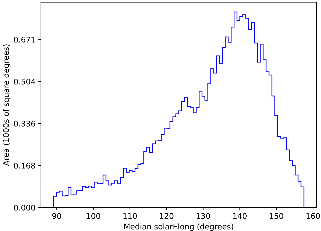
ddf_acor_sf20_lsf0_lsr0_v3.4_10yrs All sky g band: Median solarElong
