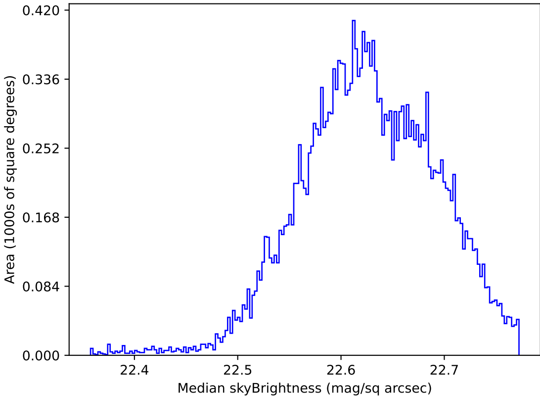
ddf_acor_sf20_lsf0_lsr0_v3.4_10yrs Yr 1 u band: Median skyBrightness
