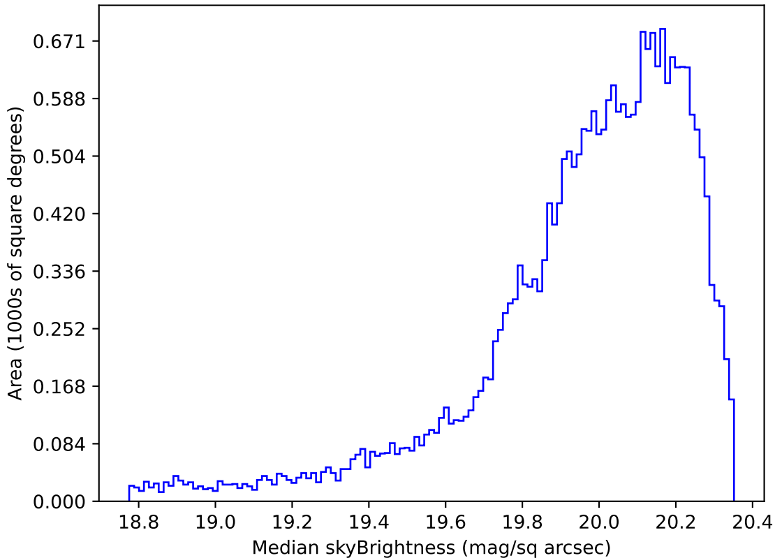
ddf_acor_sf20_lsf0_lsr0_v3.4_10yrs Yr 1 i band: Median skyBrightness
