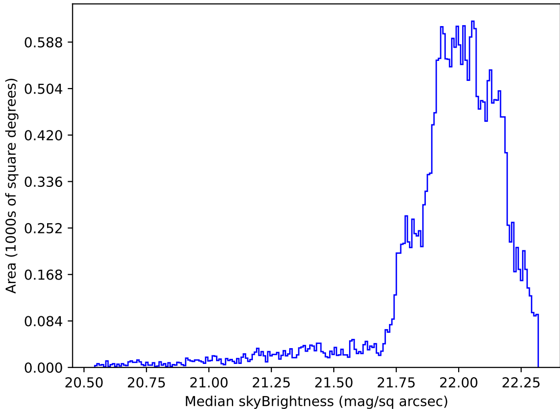
ddf_acor_sf20_lsf0_lsr0_v3.4_10yrs Yr 1 g band: Median skyBrightness
