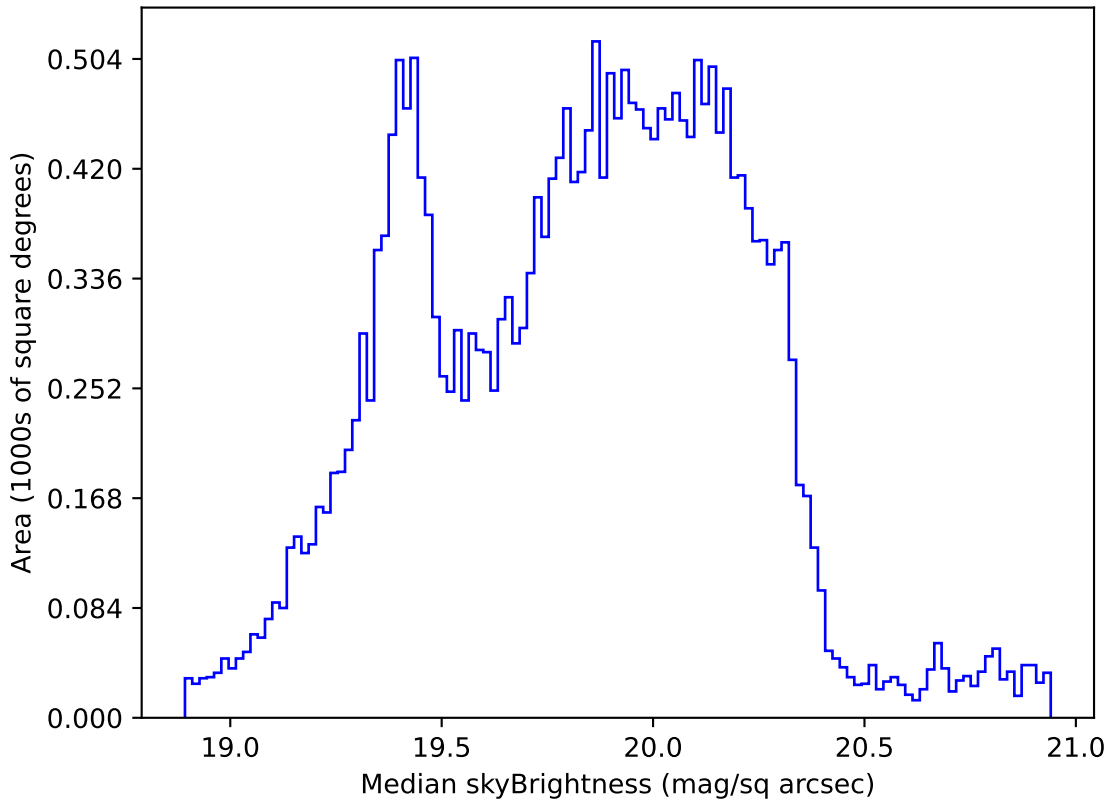
ddf_acor_sf20_lsf0_lsr0_v3.4_10yrs Yr 1 all bands: Median skyBrightness
