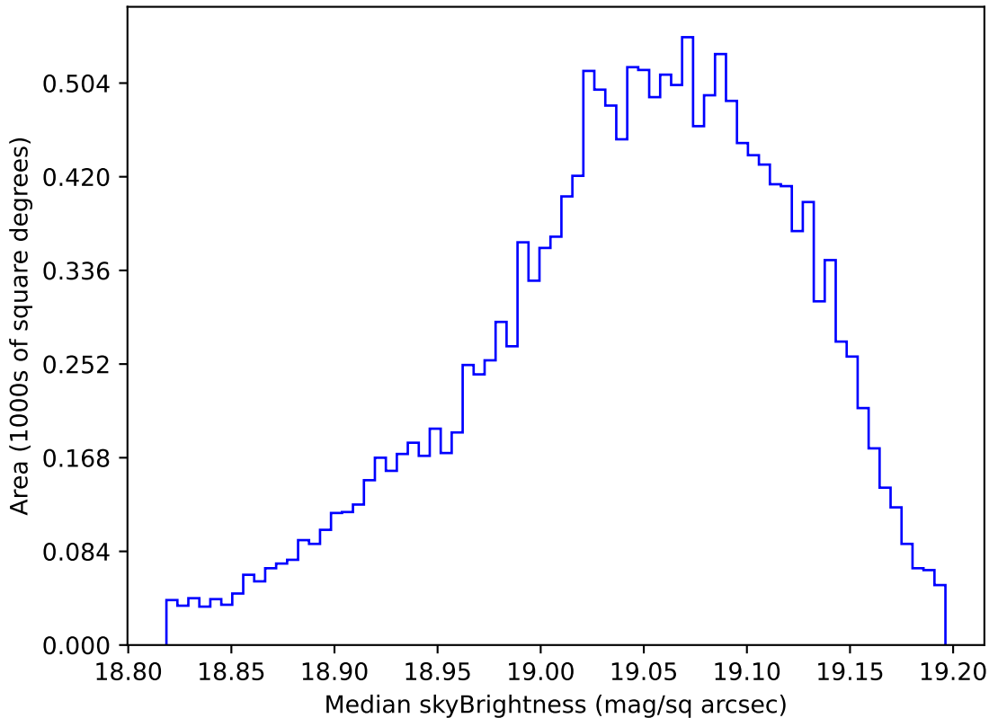
ddf_acor_sf20_lsf0_lsr0_v3.4_10yrs WFD z band: Median skyBrightness
