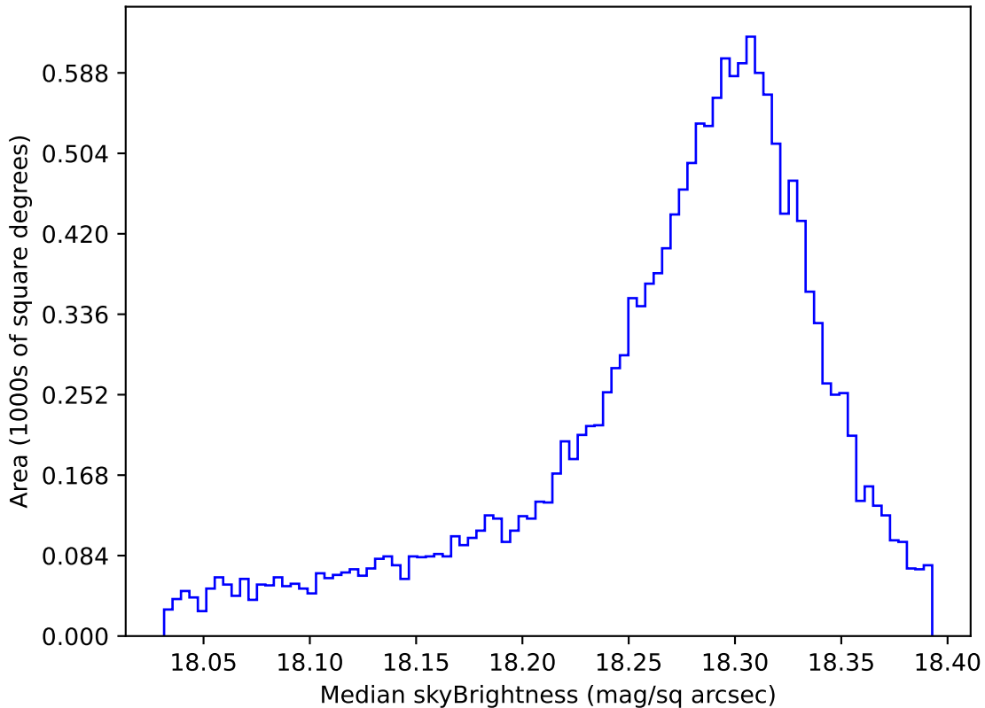
ddf_acor_sf20_ls0_lsr0_v3.4_10yrs WFD y band: Median skyBrightness
