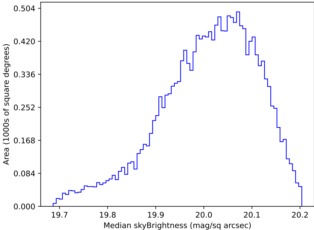
ddf_acor_sf20_lsf0_lsr0_v3.4_10yrs WFD i band: Median skyBrightness
