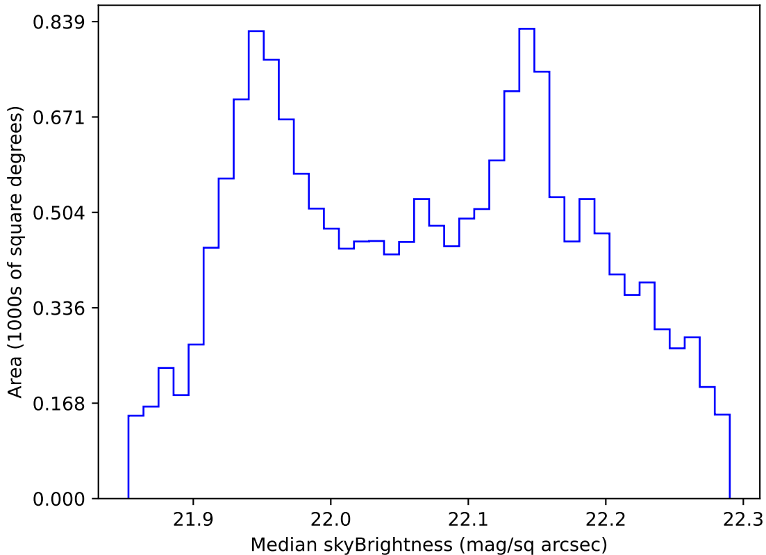
ddf_acor_sf20_ls0_lsr0_v3.4_10yrs WFD g band: Median skyBrightness
