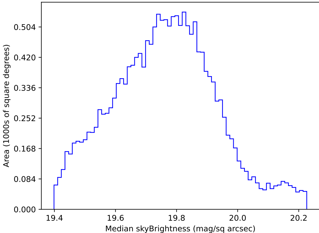
ddf_acor_sf20_lsf0_lsr0_v3.4_10yrs WFD all bands: Median skyBrightness
