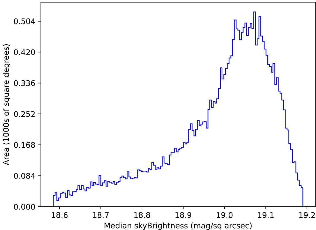
ddf_acor_sf20_lsf0_lsr0_v3.4_10yrs All sky z band: Median skyBrightness
