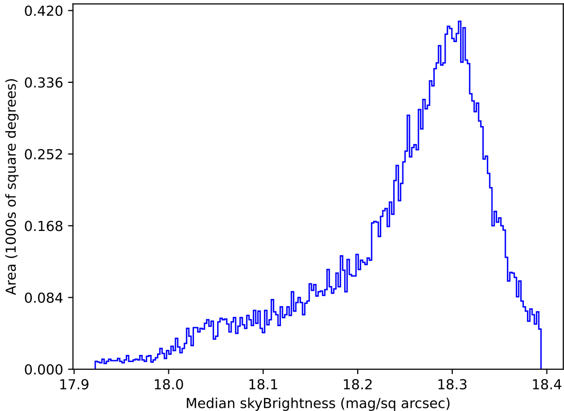
ddf_acor_sf20_lsf0_lsr0_v3.4_10yrs All sky y band: Median skyBrightness
