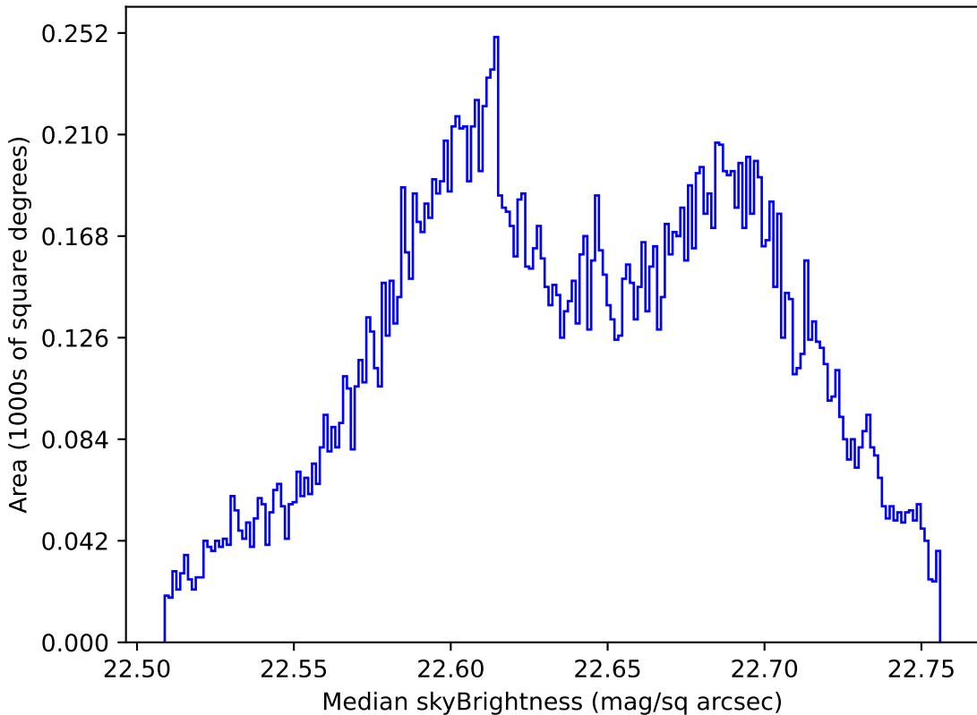
ddf_acor_sf20_lsf0_lsr0_v3.4_10yrs All sky u band: Median skyBrightness
