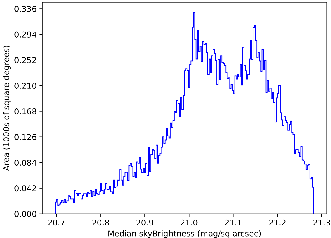
ddf_acor_sf20_lsf0_lsr0_v3.4_10yrs All sky r band: Median skyBrightness
