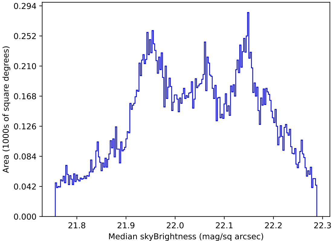
ddf_acor_sf20_lsf0_lsr0_v3.4_10yrs All sky g band: Median skyBrightness
