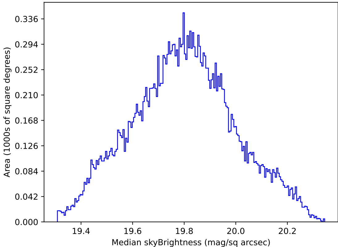
ddf_acor_sf20_lsflsr0_v3.4_10yrs All sky all bands: Median skyBrightness
