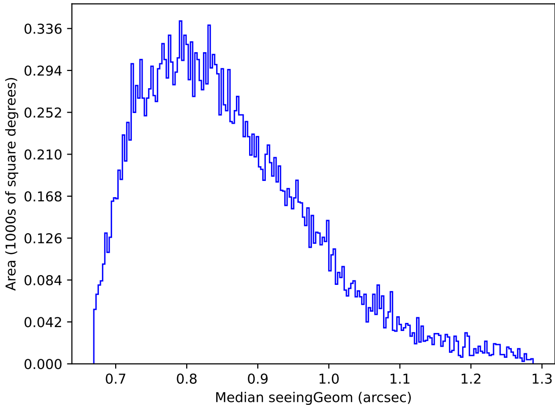
ddf_acor_sf20_lsf0_lsr0_v3.4_10yrs Yr 1 z band: Median seeingGeom
