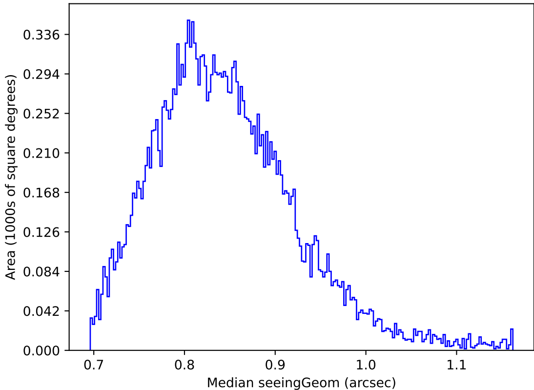
ddf_acor_sf20_lsf0_lsr0_v3.4_10yrs Yr 1 y band: Median seeingGeom
