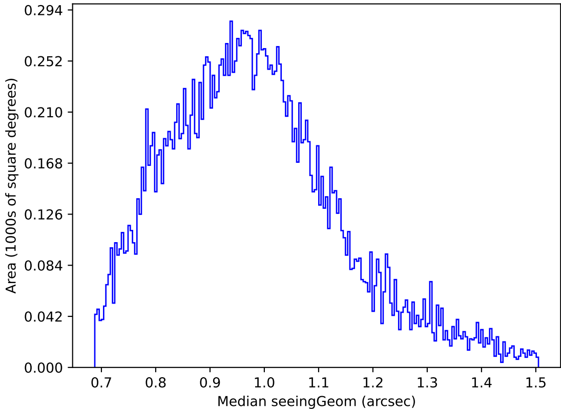
ddf_acor_sf20_lsf0_lsr0_v3.4_10yrs Yr 1 u band: Median seeingGeom
