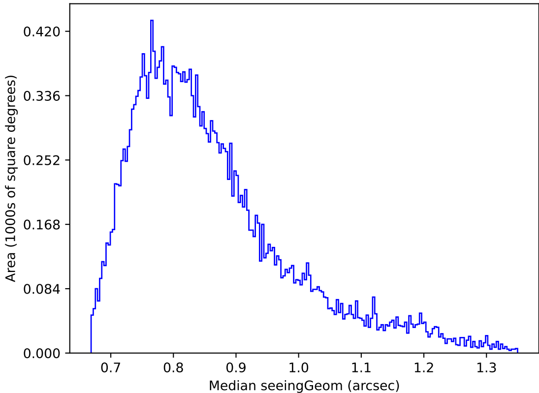
ddf_acor_sf20_lsf0_lsr0_v3.4_10yrs Yr 1 r band: Median seeingGeom
