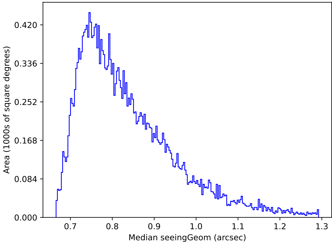
ddf_acor_sf20_lsf0_lsr0_v3.4_10yrs Yr 1 i band: Median seeingGeom
