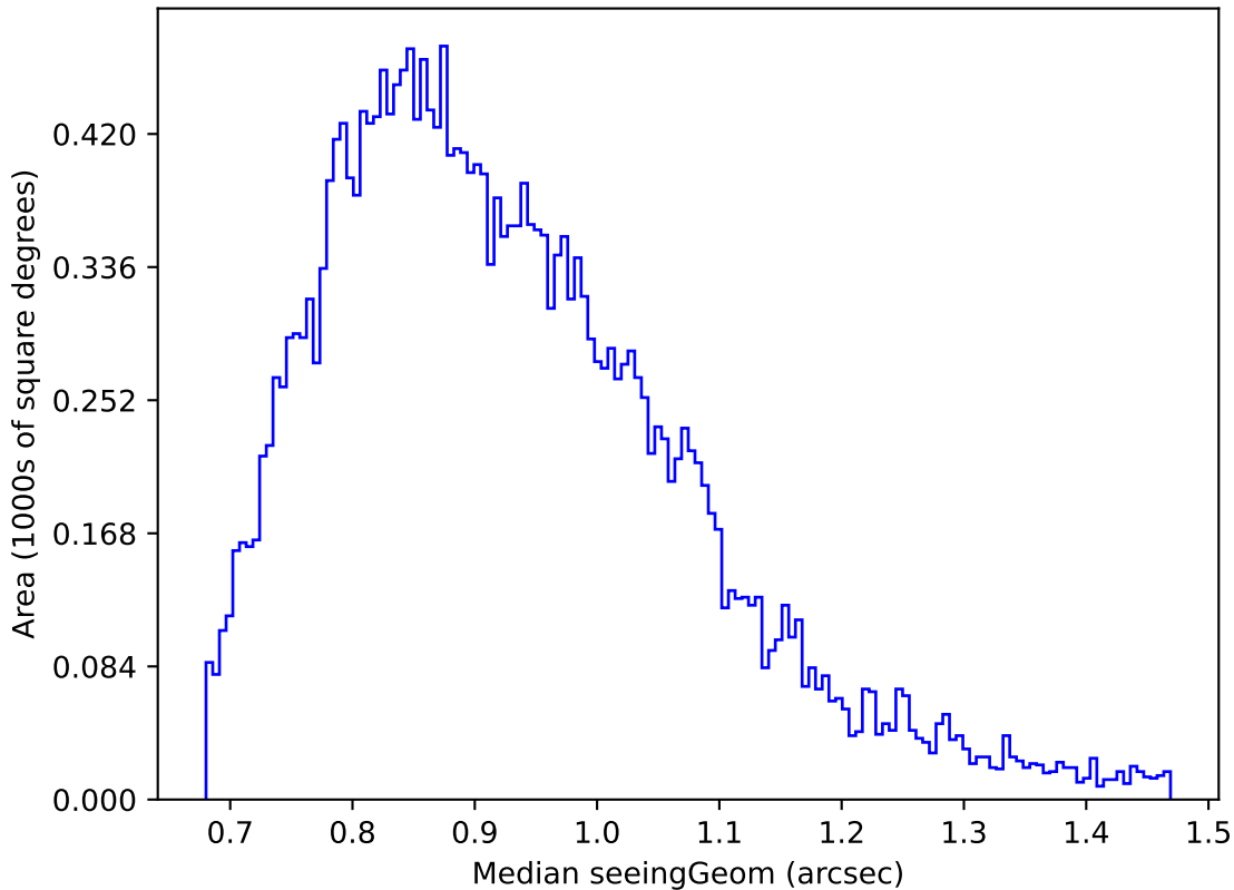
ddf_acor_sf20_lsf0_lsr0_v3.4_10yrs Yr 1 g band: Median seeingGeom
