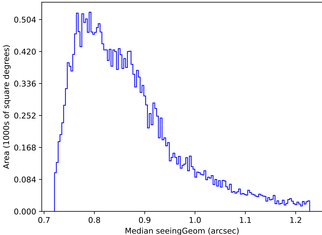
ddf_acor_sf20_lsf0_lsr0_v3.4_10yrs Yr 1 all bands: Median seeingGeom
