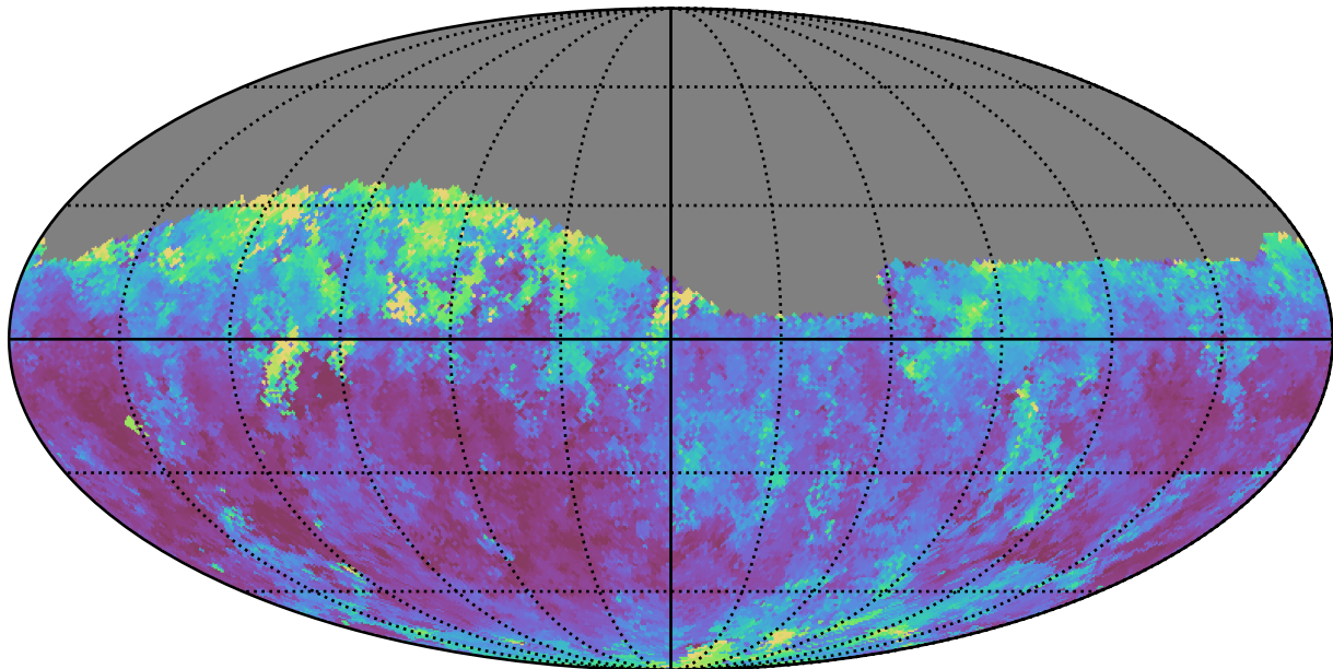
ddf_acor_sf20_lsf0_lsr0_v3.4_10yrs Yr 1 z band: Median seeingEff
