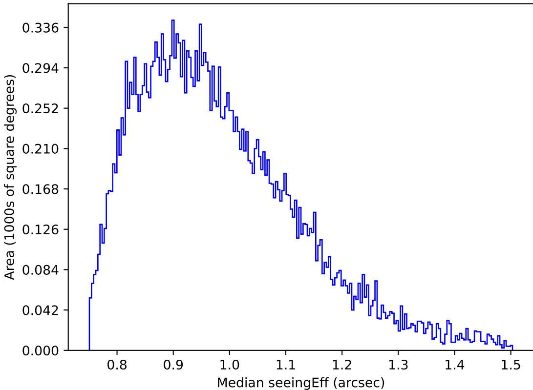
ddf_acor_sf20_lsf0_lsr0_v3.4_10yrs Yr 1 z band: Median seeingEff
