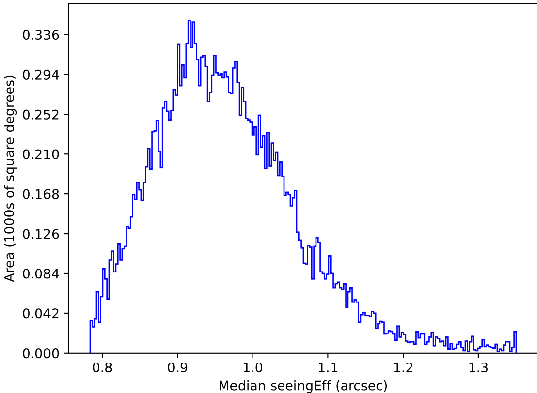
ddf_acor_sf20_lsf0_lsr0_v3.4_10yrs Yr 1 y band: Median seeingEff
