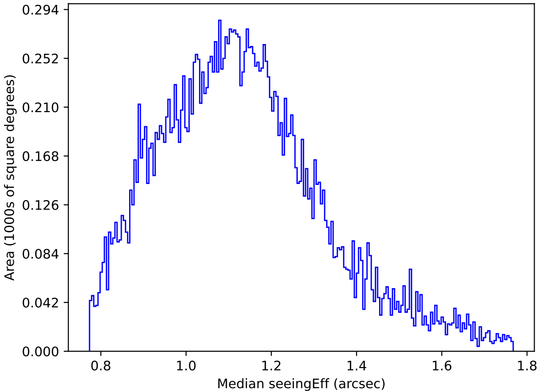
ddf_acor_sf20_lsf0_lsr0_v3.4_10yrs Yr 1 u band: Median seeingEff
