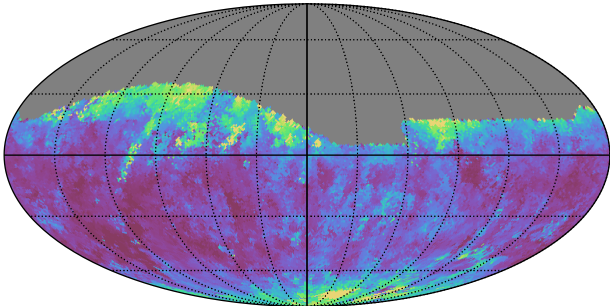
ddf_acor_sf20_lsf0_lsr0_v3.4_10yrs Yr 1 r band: Median seeingEff
