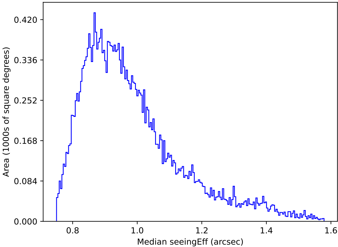
ddf_acor_sf20_lsf0_lsr0_v3.4_10yrs Yr 1 r band: Median seeingEff
