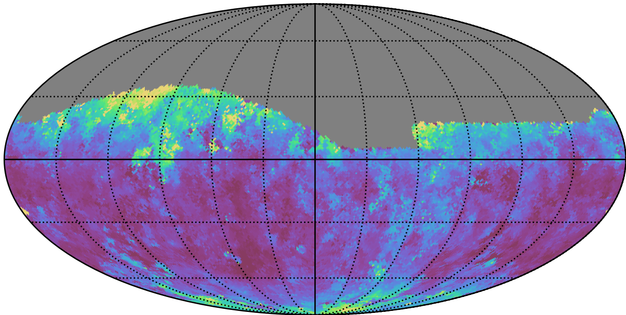
ddf_acor_sf20_lsf0_lsr0_v3.4_10yrs Yr 1 i band: Median seeingEff
