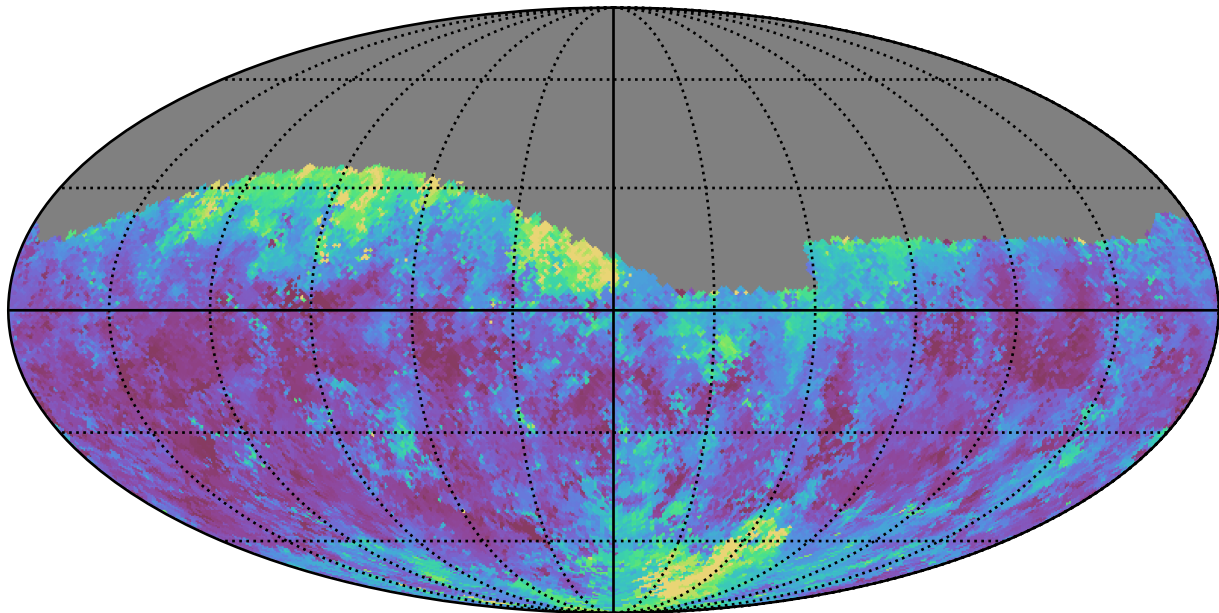
ddf_acor_sf20_lsf0_lsr0_v3.4_10yrs Yr 1 g band: Median seeingEff
