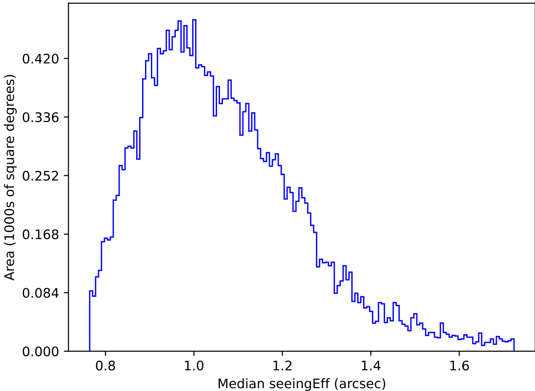
ddf_acor_sf20_lsf0_lsr0_v3.4_10yrs Yr 1 g band: Median seeingEff
