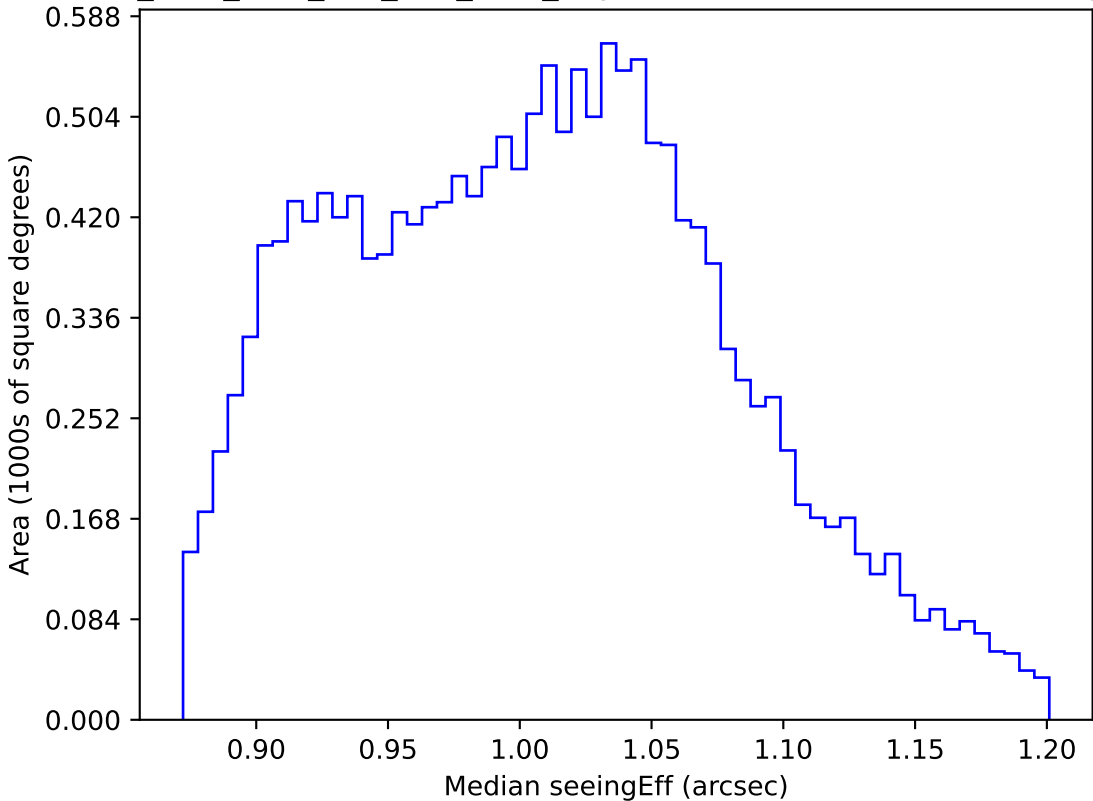
ddf_acor_sf20_lsf0_lsr0_v3.4_10yrs WFD z band: Median seeingEff
