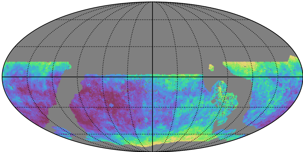
ddf_acor_sf20_lsf0_lsr0_v3.4_10yrs WFD y band: Median seeingEff
