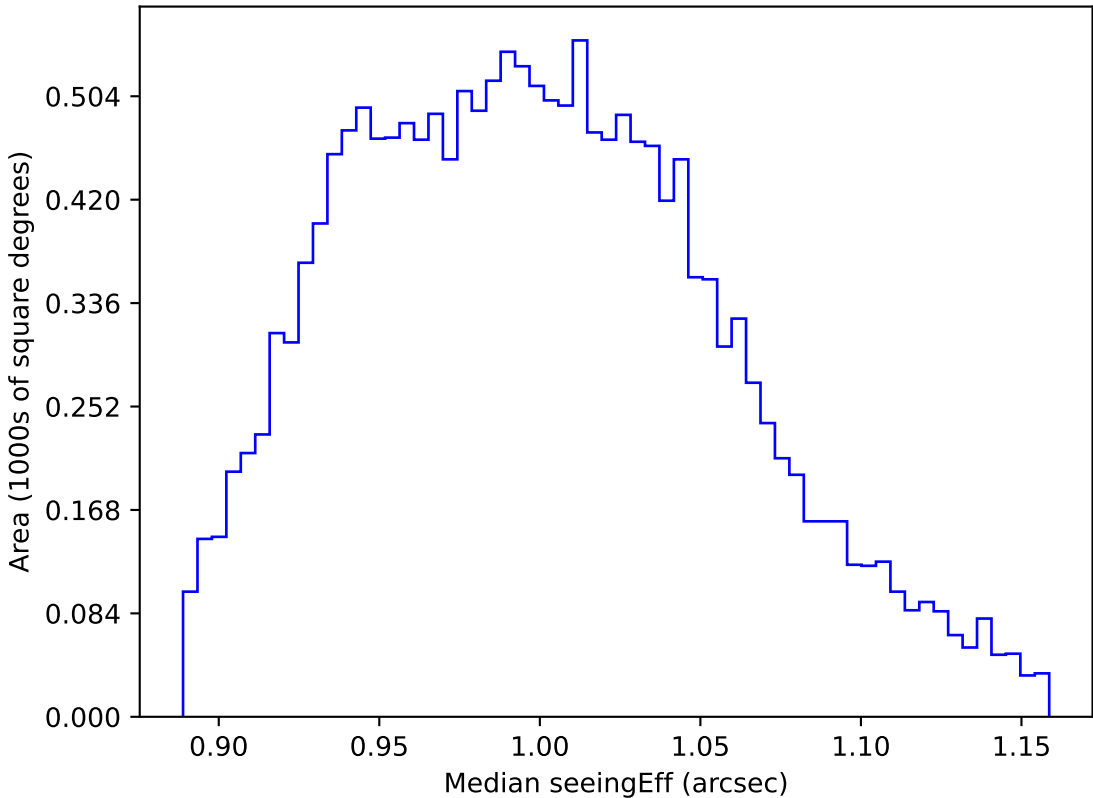
ddf_acor_sf20_lsf0_lsr0_v3.4_10yrs WFD y band: Median seeingEff
