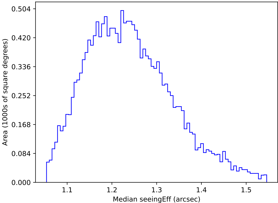
ddf_acor_sf20_lsf0_lsr0_v3.4_10yrs WFD u band: Median seeingEff
