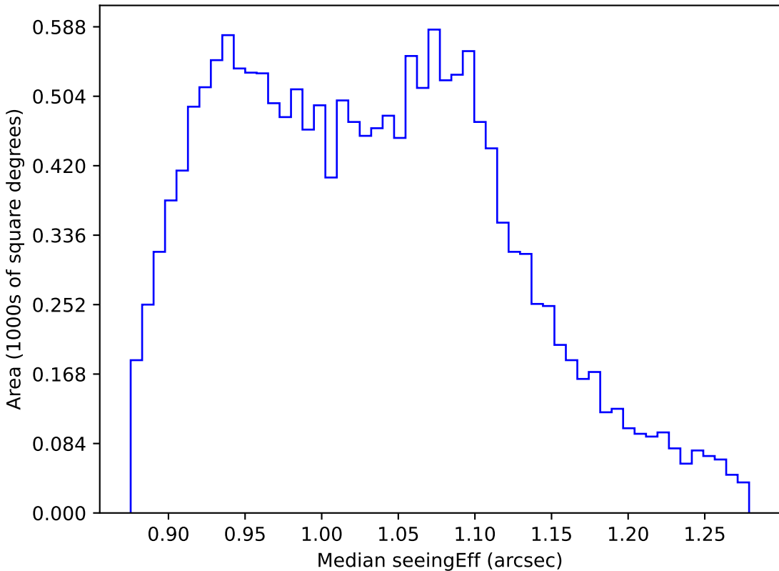
ddf_acor_sf20_lsf0_lsr0_v3.4_10yrs WFD r band: Median seeingEff
