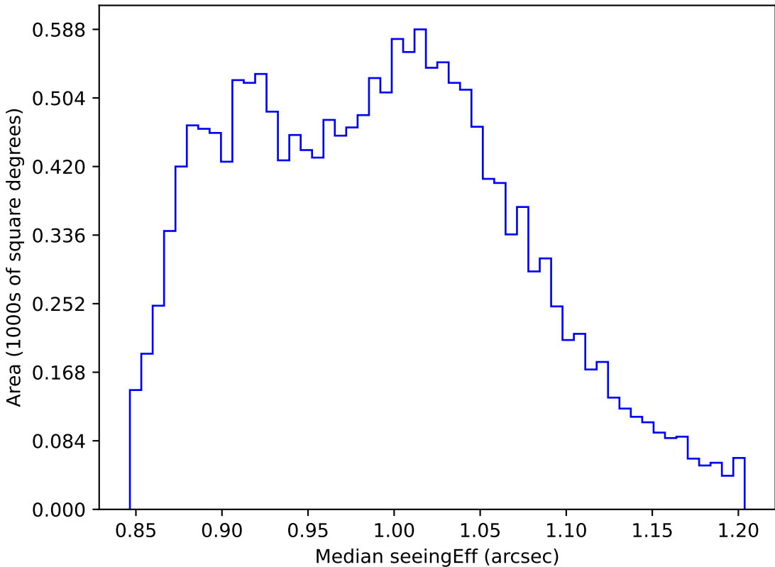
ddf_acor_sf20_lsf0_lsr0_v3.4_10yrs WFD i band: Median seeingEff
