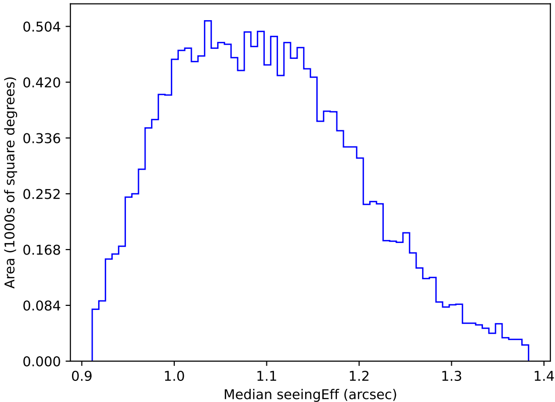
ddf_acor_sf20_lsf0_lsr0_v3.4_10yrs WFD g band: Median seeingEff
