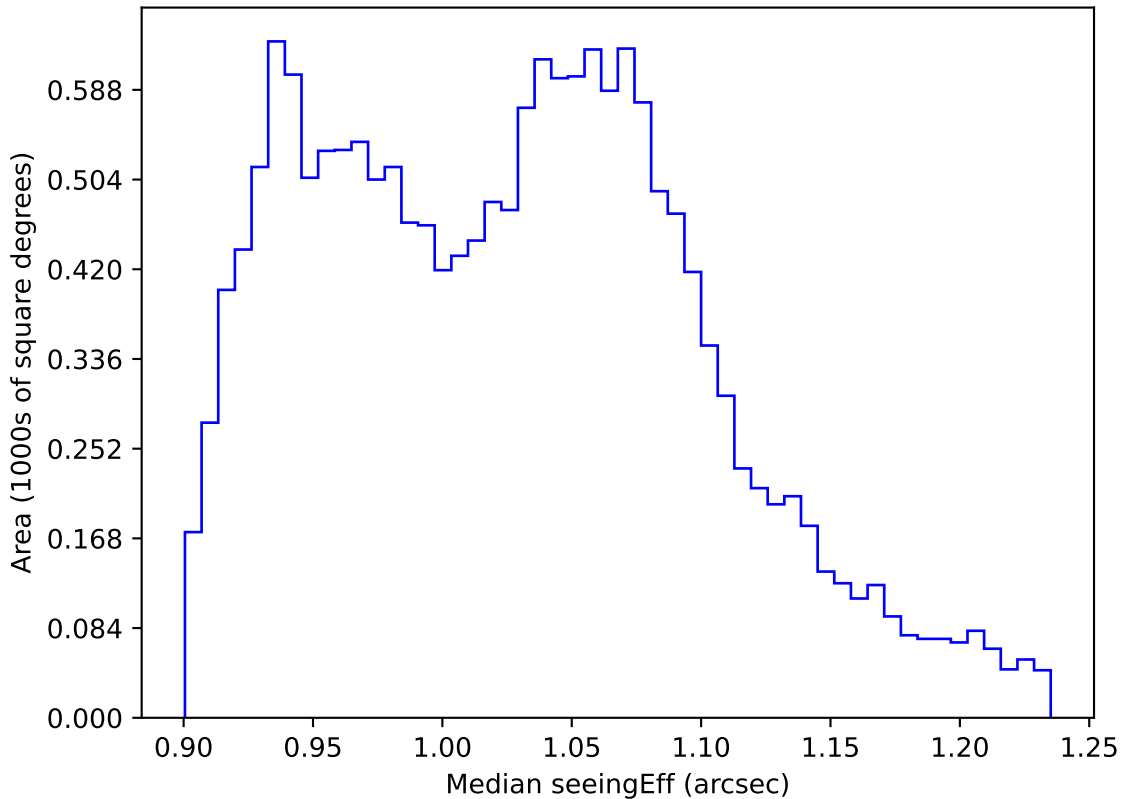
ddf_acor_sf20_lsf0_lsr0_v3.4_10yrs WFD all bands: Median seeingEff
