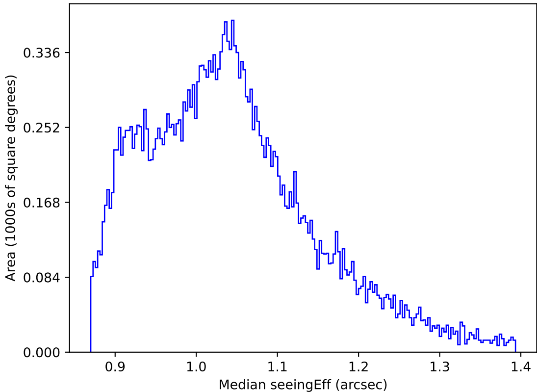
ddf_acor_sf20_ls0_lsr0_v3.4_10yrs All sky z band: Median seeingEff
