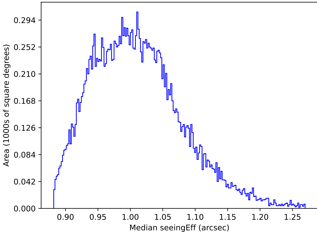
ddf_acor_sf20_lsf0_lsr0_v3.4_10yrs All sky y band: Median seeingEff
