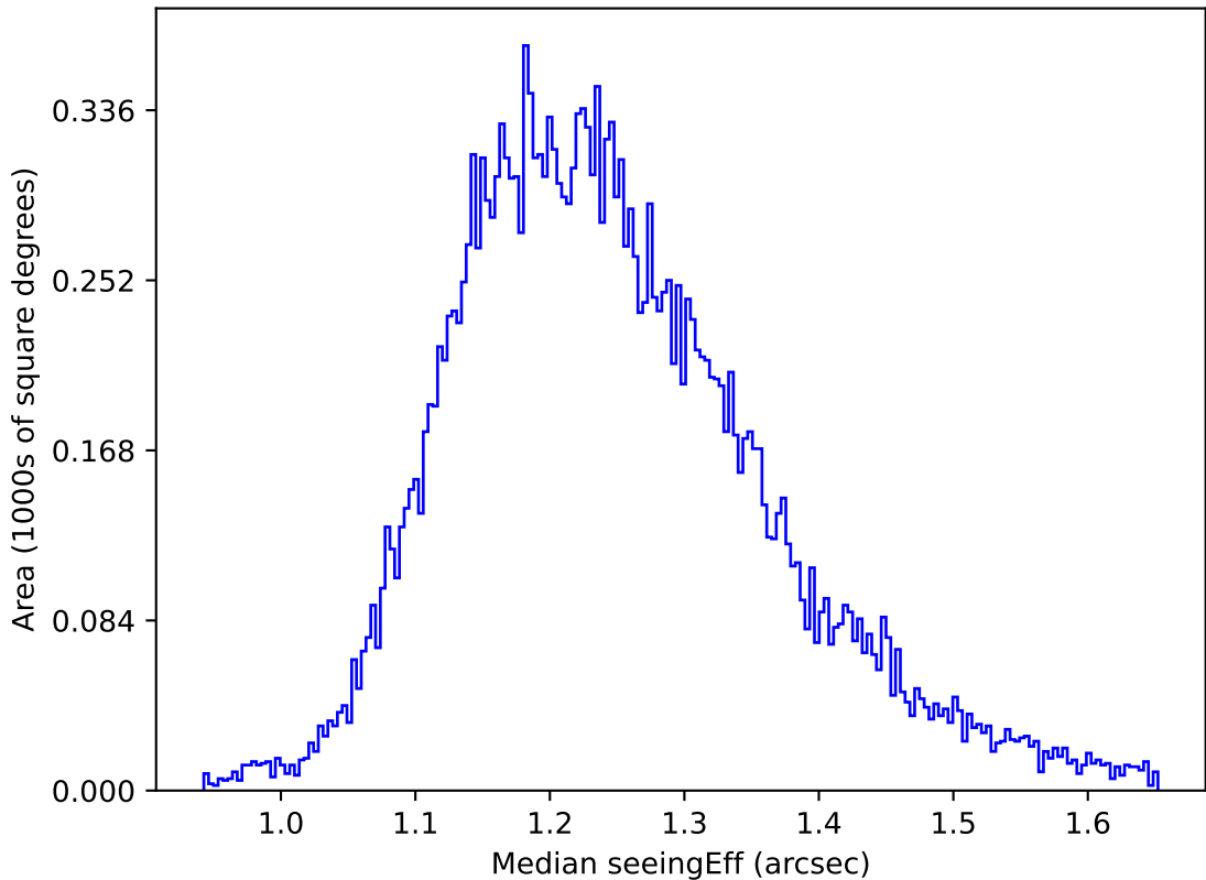
ddf_acor_sf20_lsf0_lsr0_v3.4_10yrs All sky u band: Median seeingEff
