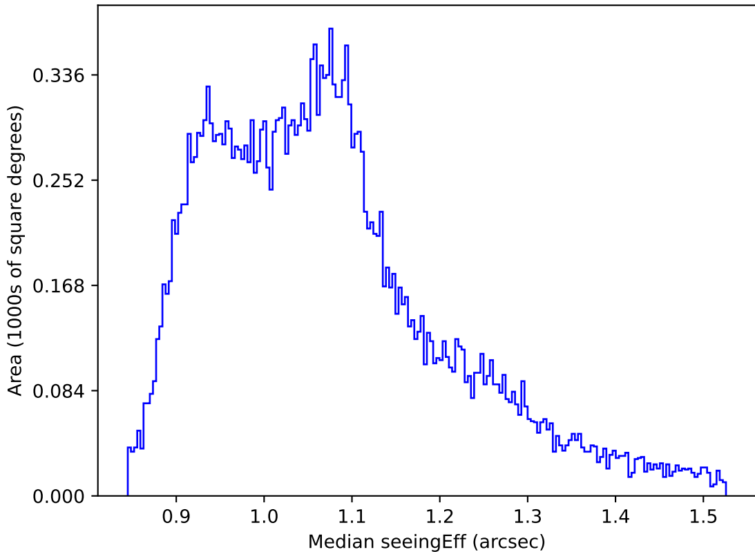
ddf_acor_sf20_ls0_lsr0_v3.4_10yrs All sky r band: Median seeingEff
