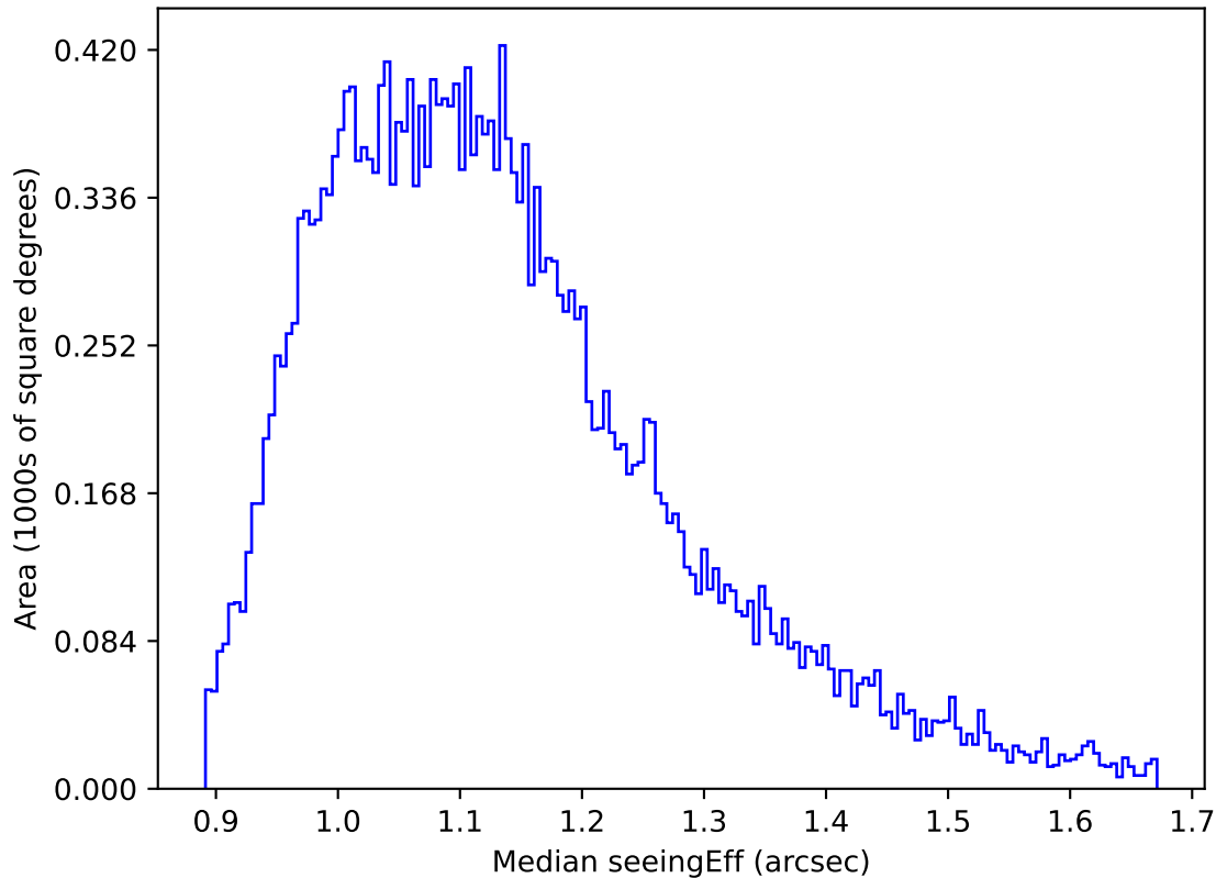
ddf_acor_sf20_lsf0_lsr0_v3.4_10yrs All sky g band: Median seeingEff
